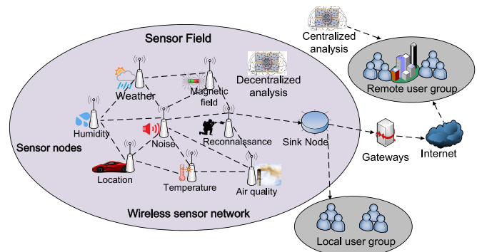
Fig. 16. An example framework for WSN data collection and (centralized and decentralized) analysis.
