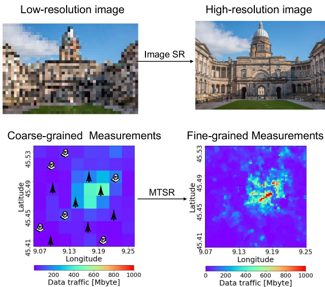
Fig. 11. Illustration of the image super-resolution (SR) principle (above) and the mobile traffic super-resolution (MTSR) technique (below). Figure adapted from [218].
